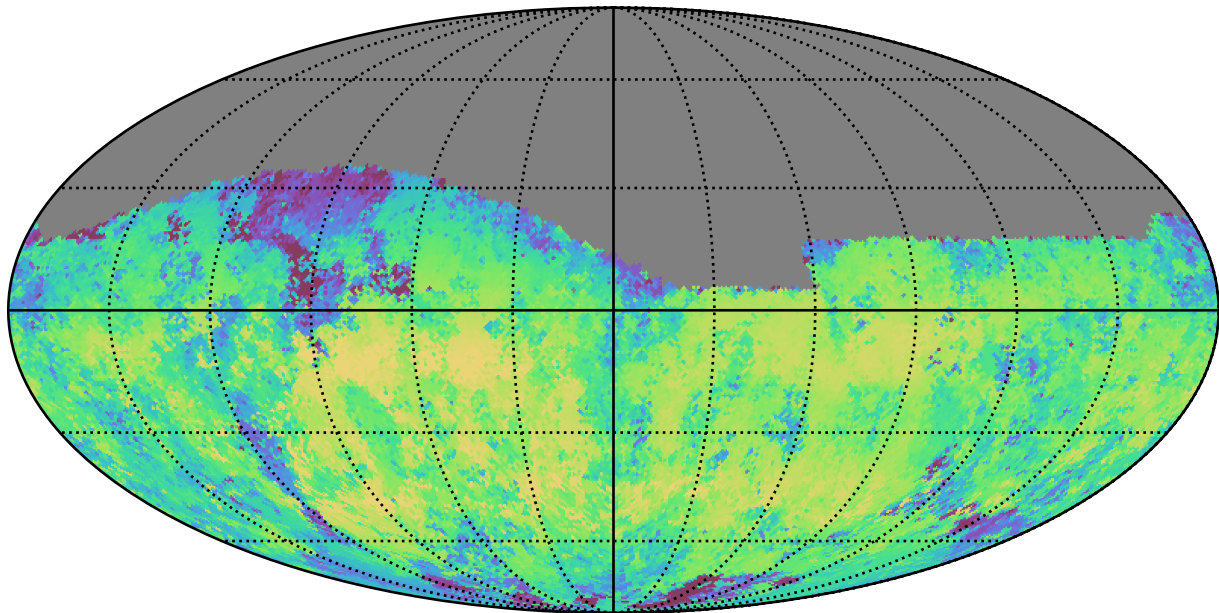
ddf_loaded_fl8_v3.4_10yrs Yr 1 i band: Median skyBrightness
