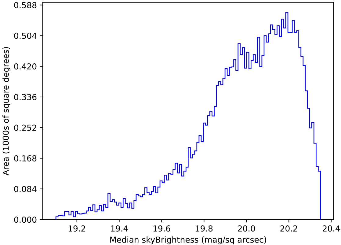
ddf_loaded_fl8_v3.4_10yrs Yr 1 i band: Median skyBrightness
