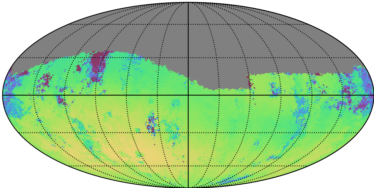
ddf_loaded_fl8_v3.4_10yrs Yr 1 g band: Median skyBrightness
