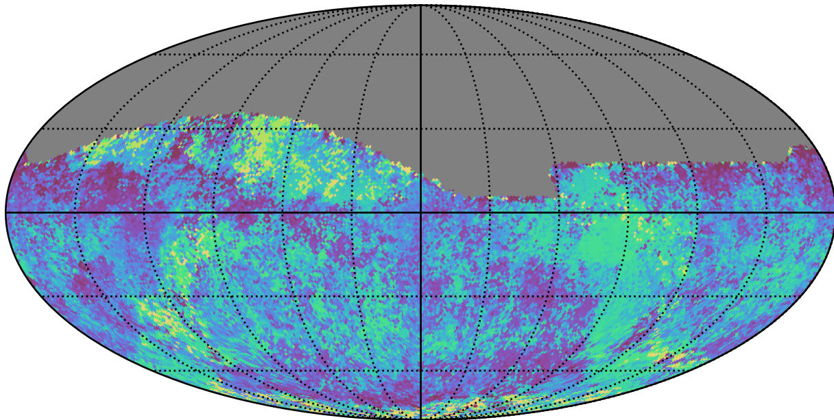
ddf_loaded_fl8_v3.4_10yrs Yr 1 all bands: Median skyBrightness
