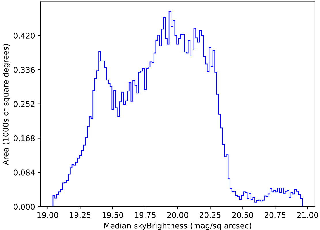
ddf_loaded_fl8_v3.4_10yrs Yr 1 all bands: Median skyBrightness
