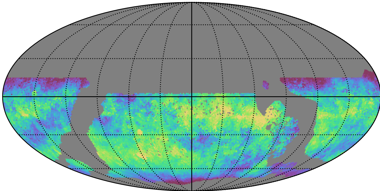
ddf_loaded_fl8_v3.4_10yrs WFD z band: Median skyBrightness
