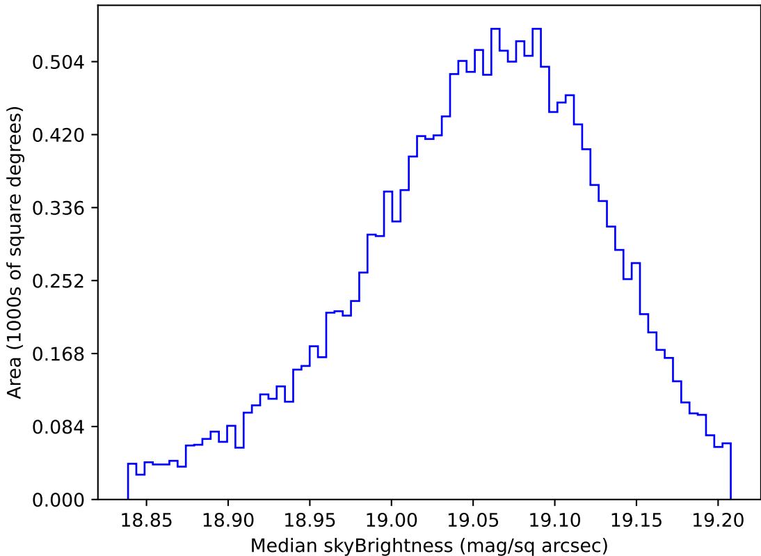
ddf_loaded_fl8_v3.4_10yrs WFD z band: Median skyBrightness
