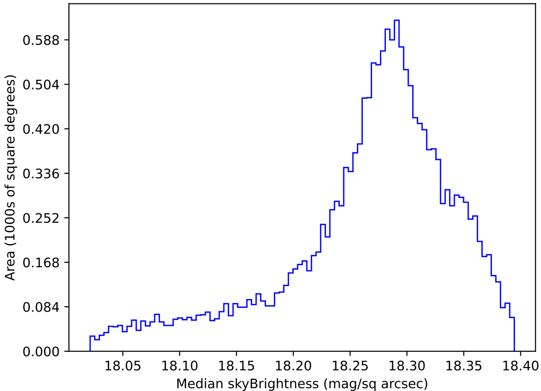
ddf_loaded_fl8_v3.4_10yrs WFD y band: Median skyBrightness
