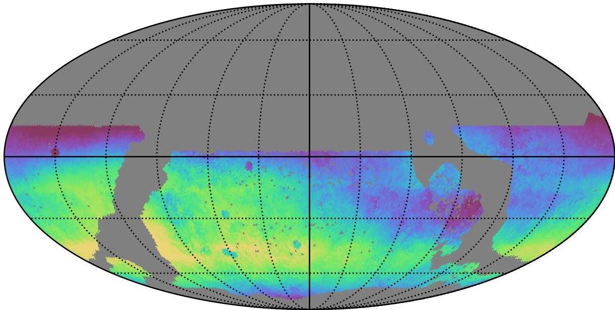
ddf_loaded_fl8_v3.4_10yrs WFD u band: Median skyBrightness
