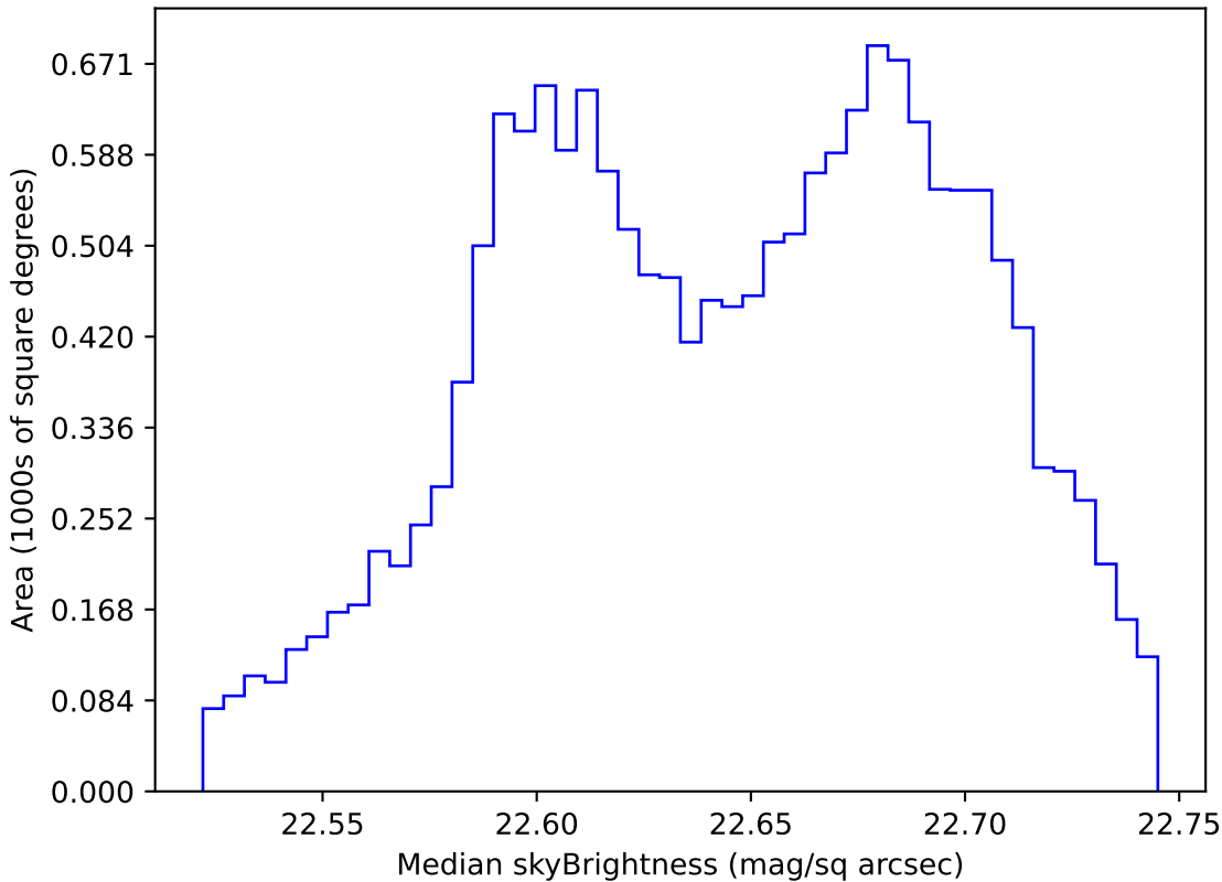
ddf_loaded_fl8_v3.4_10yrs WFD u band: Median skyBrightness
