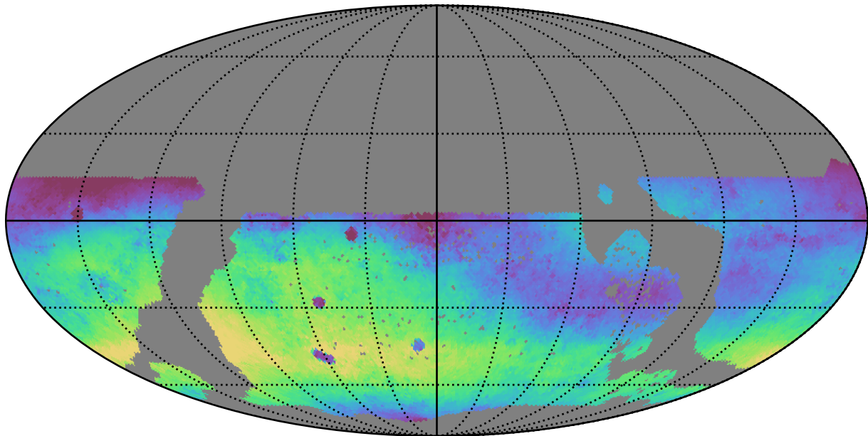
ddf_loaded_fl8_v3.4_10yrs WFD r band: Median skyBrightness
