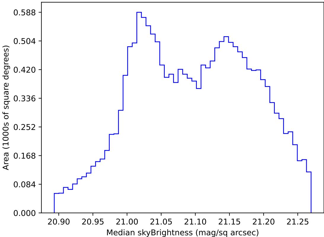
ddf_loaded_fl8_v3.4_10yrs WFD r band: Median skyBrightness
