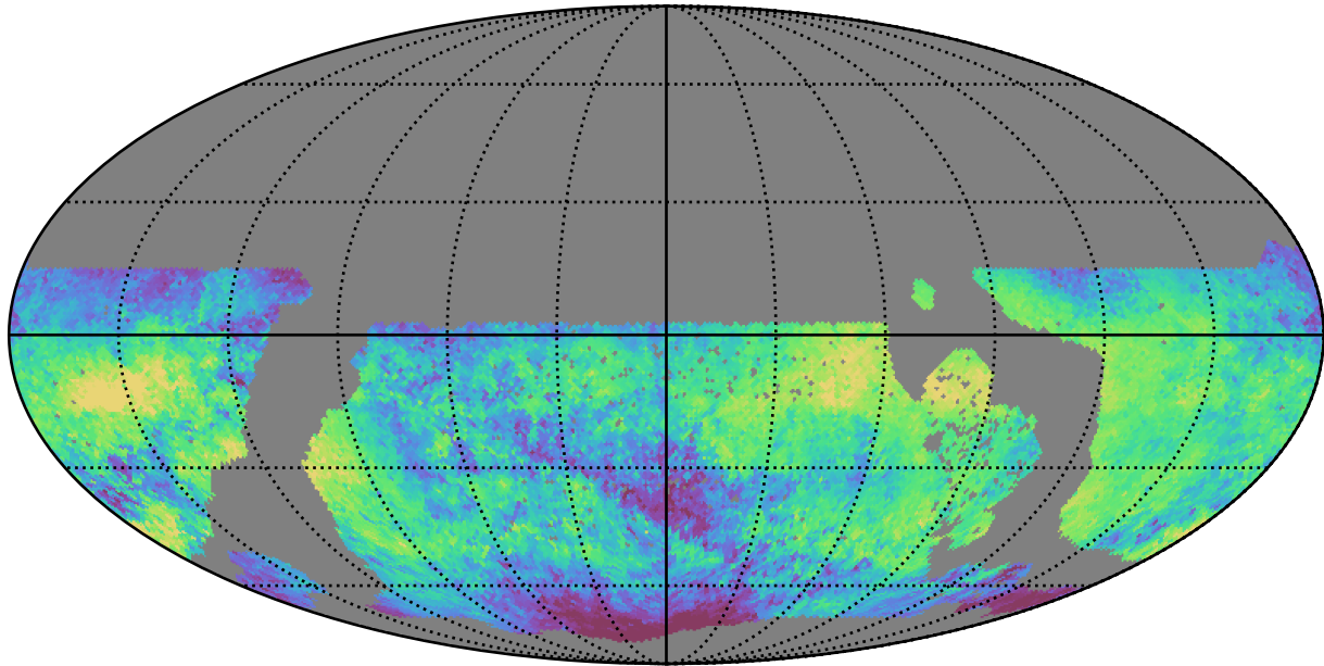
ddf_loaded_fl8_v3.4_10yrs WFD i band: Median skyBrightness
