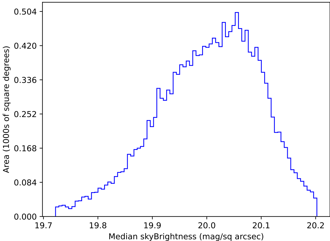
ddf_loaded_fl8_v3.4_10yrs WFD i band: Median skyBrightness
