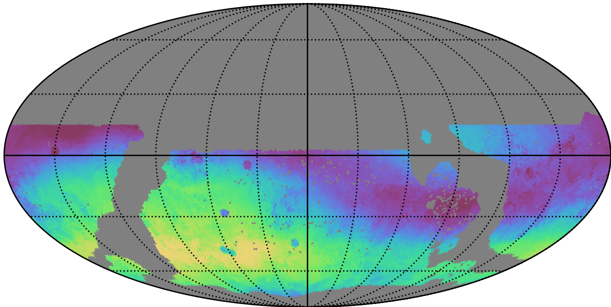
ddf_loaded_fl8_v3.4_10yrs WFD g band: Median skyBrightness
