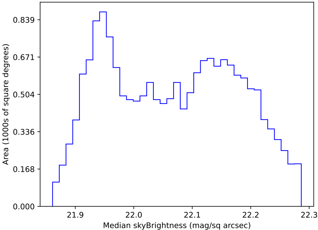
ddf_loaded_fl8_v3.4_10yrs WFD g band: Median skyBrightness
