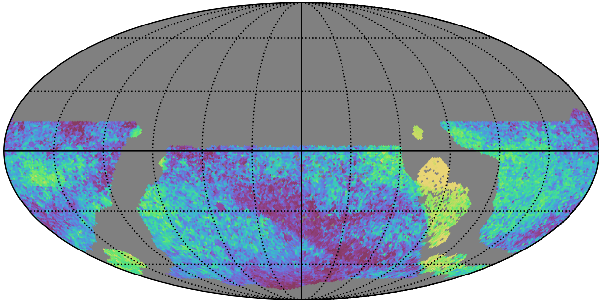
ddf_loaded_fl8_v3.4_10yrs WFD all bands: Median skyBrightness
