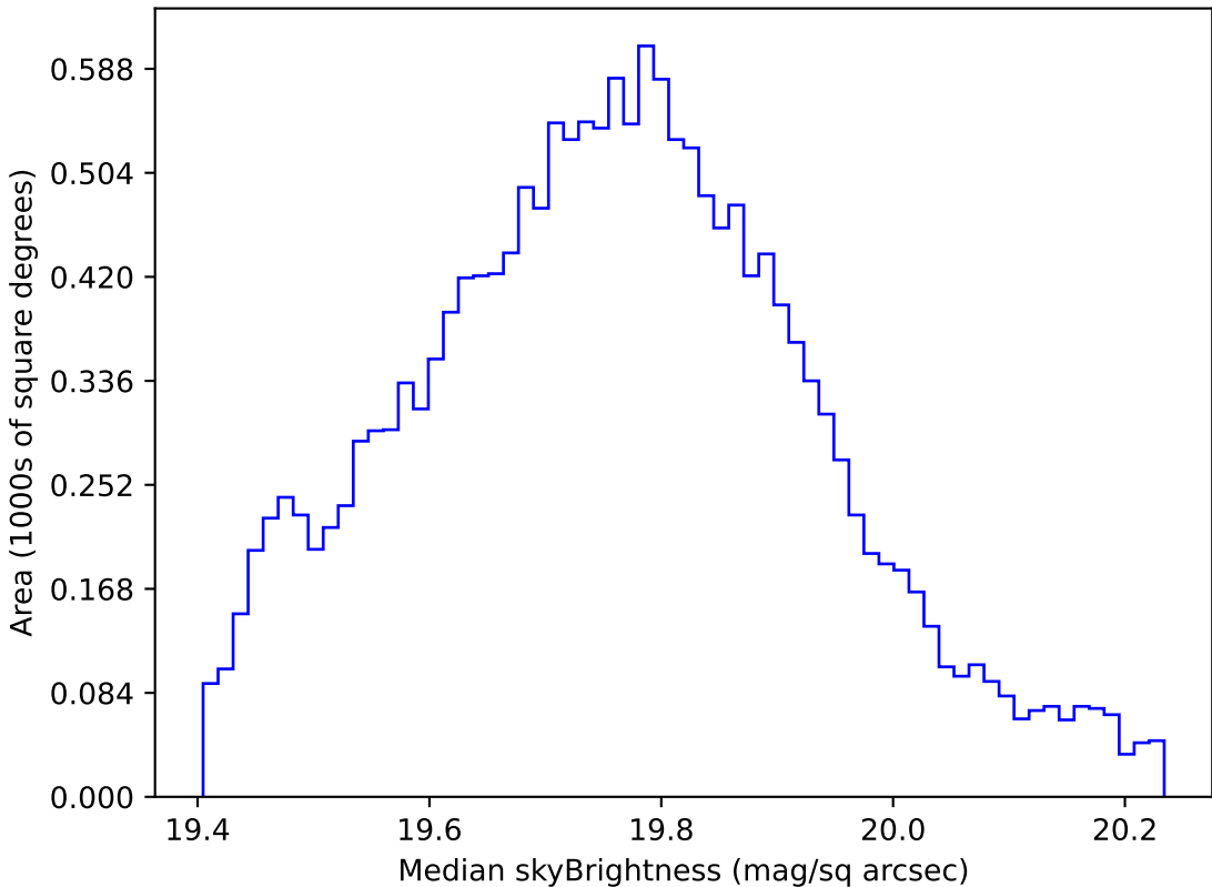
ddf_loaded_fl8_v3.4_10yrs WFD all bands: Median skyBrightness
