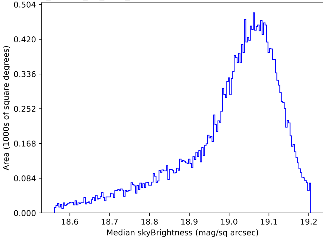
ddf_loaded_fl8_v3.4_10yrs All sky z band: Median skyBrightness
