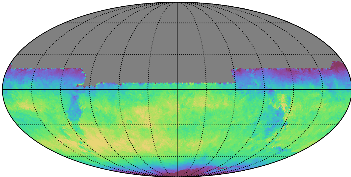
ddf_loaded_fl8_v3.4_10yrs All sky y band: Median skyBrightness
