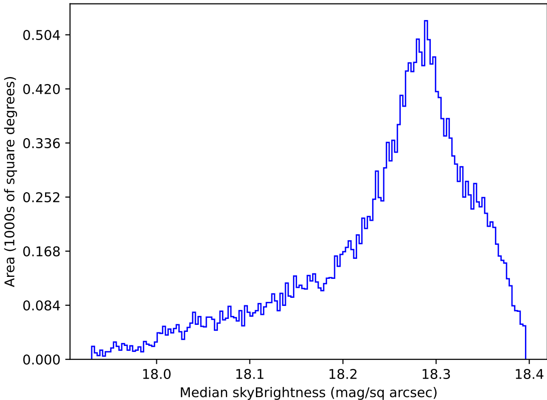
ddf_loaded_fl8_v3.4_10yrs All sky y band: Median skyBrightness
