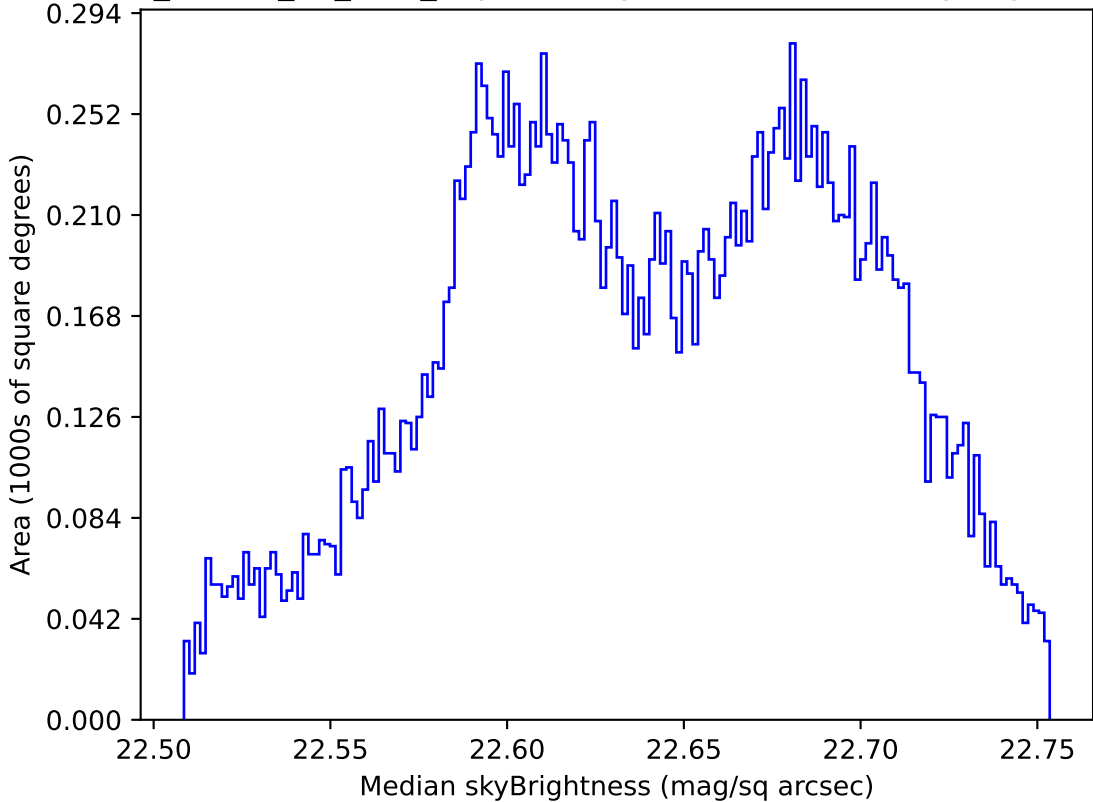
ddf_loaded_fl8_v3.4_10yrs All sky u band: Median skyBrightness
