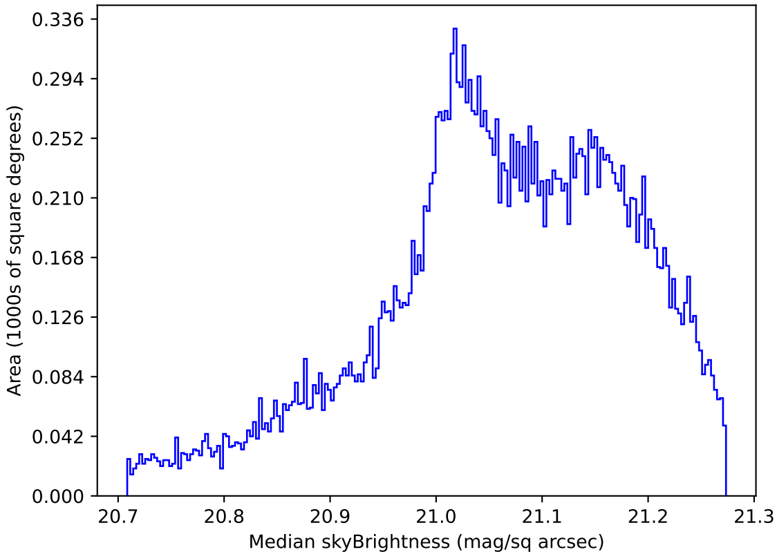
ddf_loaded_fl8_v3.4_10yrs All sky r band: Median skyBrightness
