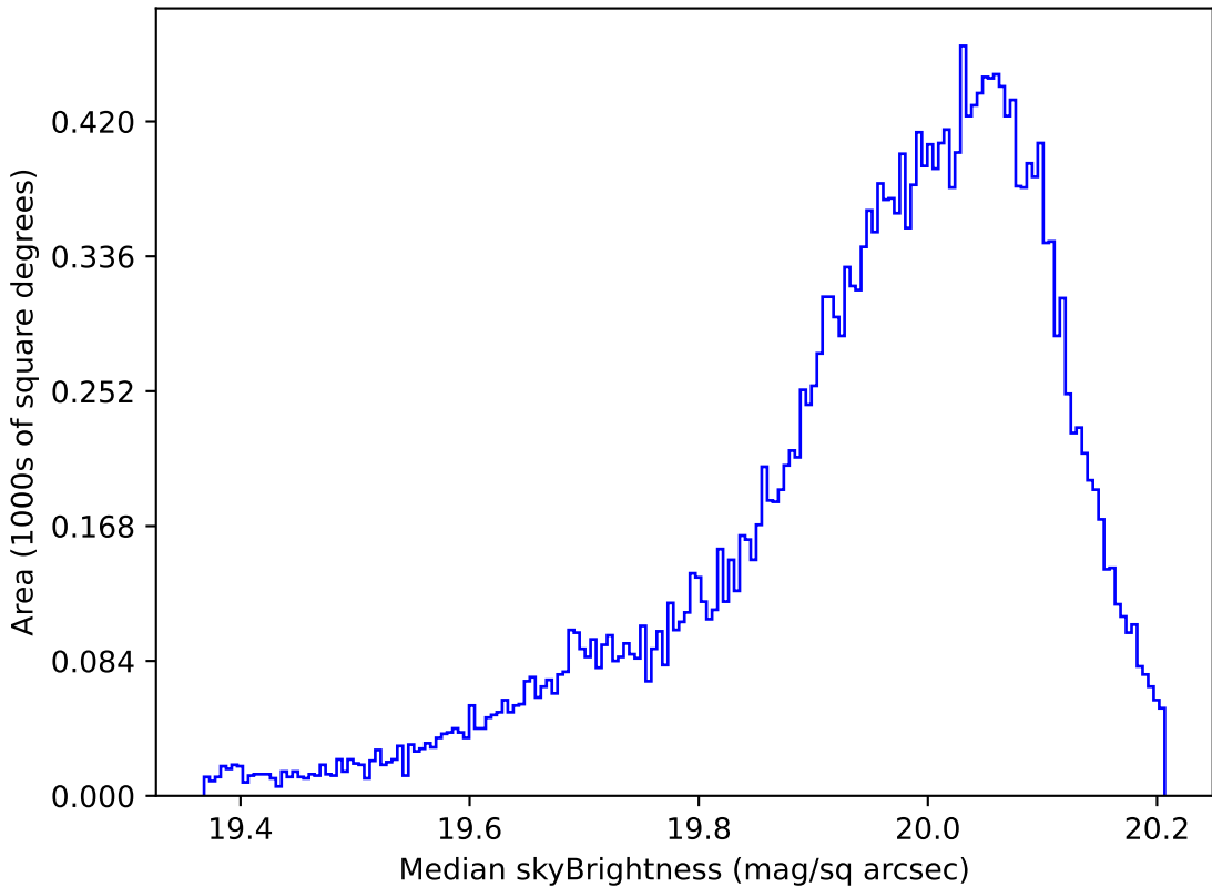
ddf_loaded_fl8_v3.4_10yrs All sky i band: Median skyBrightness
