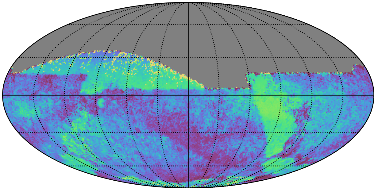
ddf_loaded_fl8_v3.4_10yrs All sky all bands: Median skyBrightness
