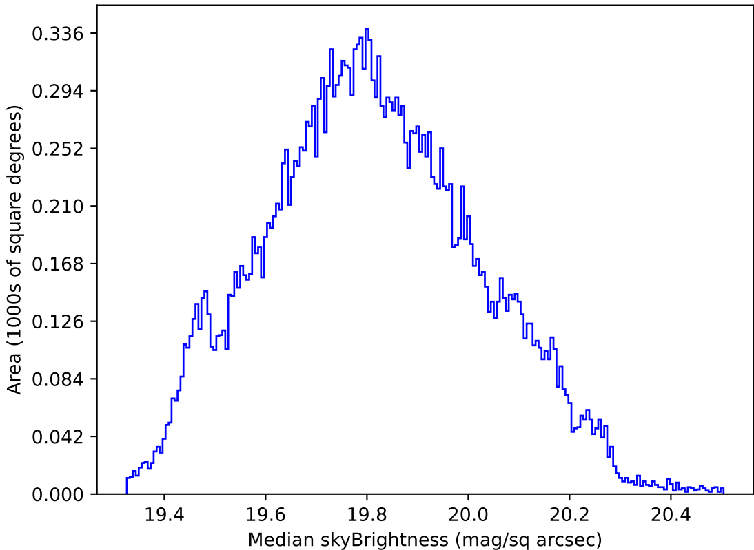
ddf_loaded_fl8_v3.4_10yrs All sky all bands: Median skyBrightness
