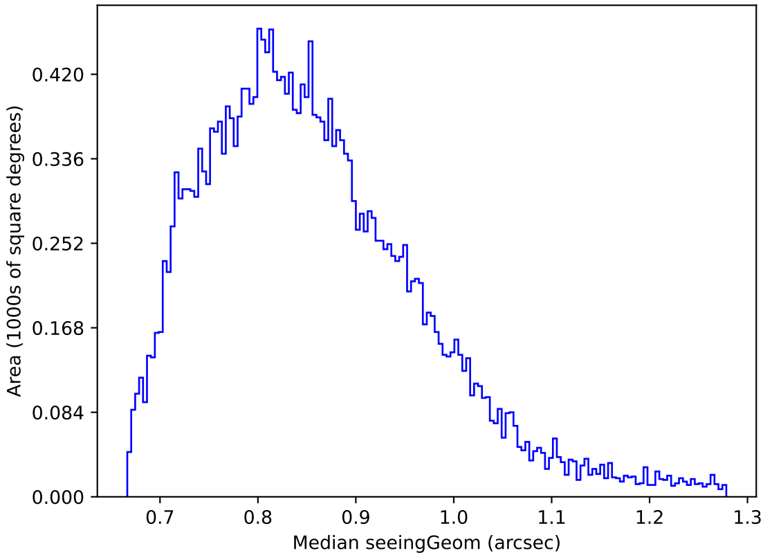
ddf_loaded_fl8_v3.4_10yrs Yr 1 z band: Median seeingGeom
