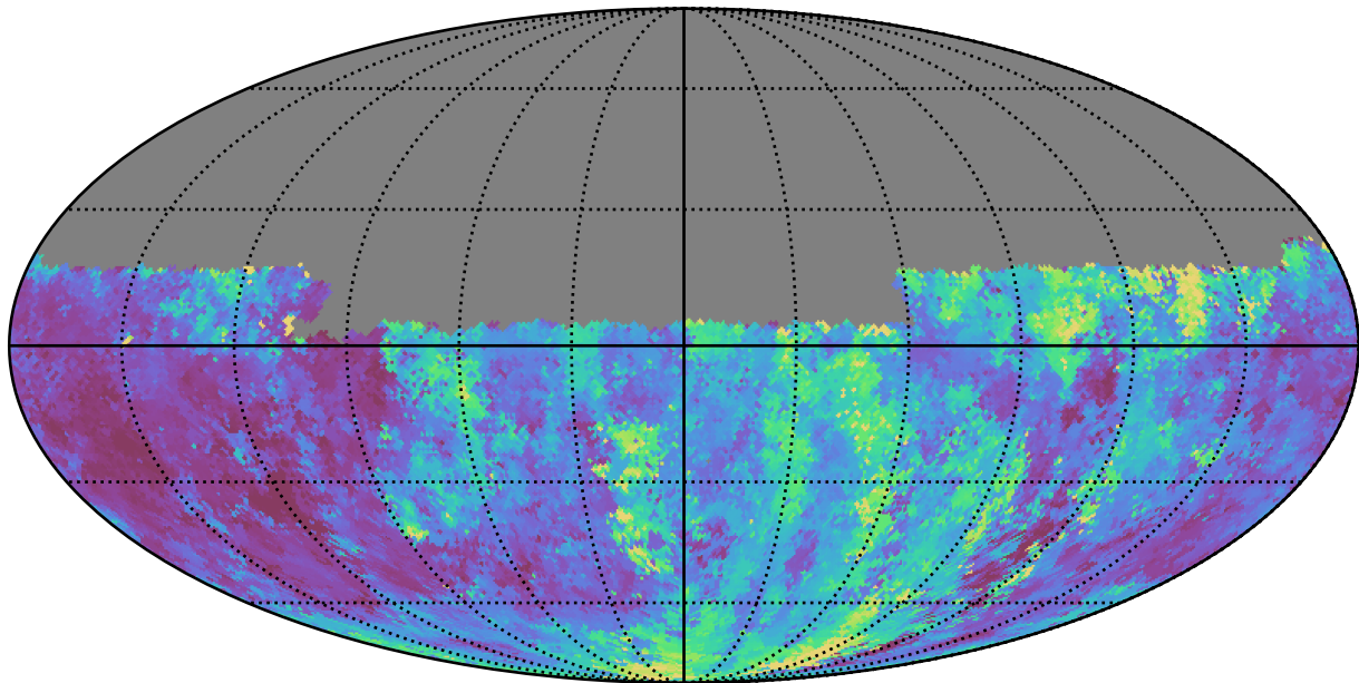
ddf_loaded_fl8_v3.4_10yrs Yr 1 u band: Median seeingGeom
