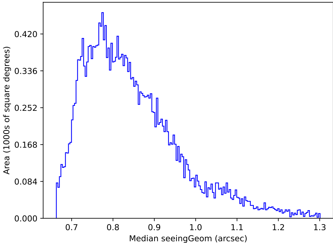
ddf_loaded_fl8_v3.4_10yrs Yr 1 r band: Median seeingGeom
