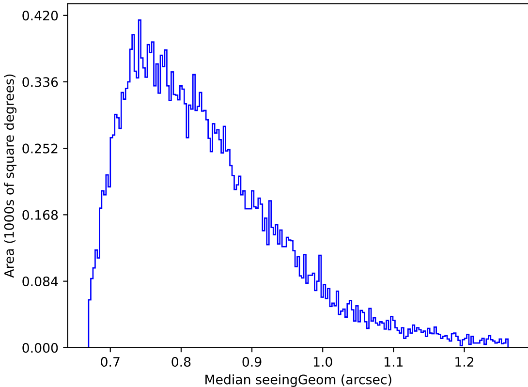
ddf_loaded_fl8_v3.4_10yrs Yr 1 i band: Median seeingGeom
