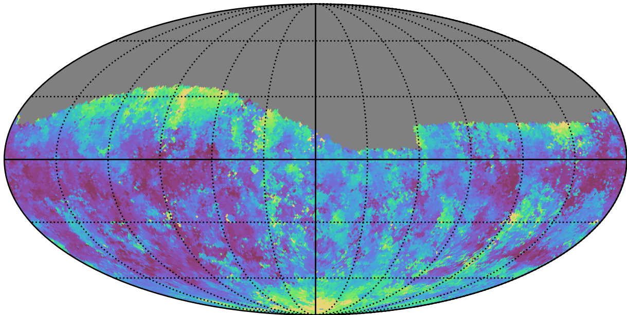
ddf_loaded_fl8_v3.4_10yrs Yr 1 g band: Median seeingGeom
