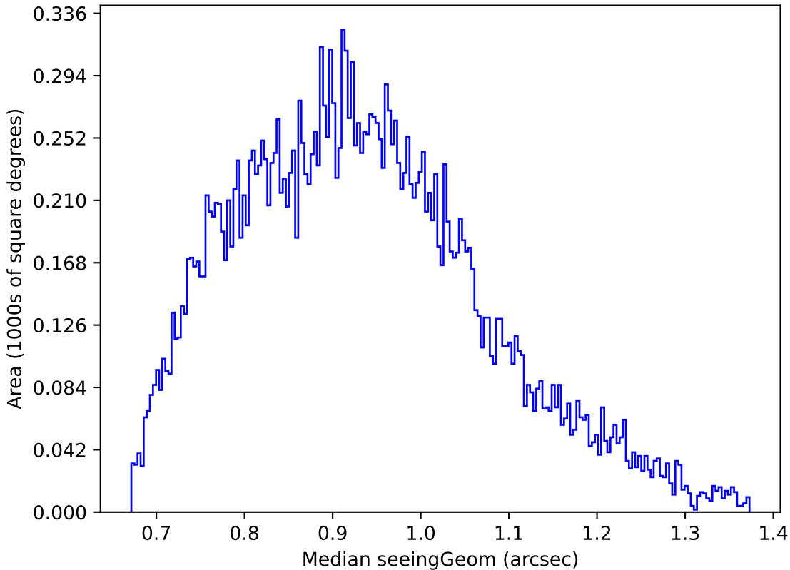
ddf_loaded_fl8_v3.4_10yrs Yr 1 g band: Median seeingGeom
