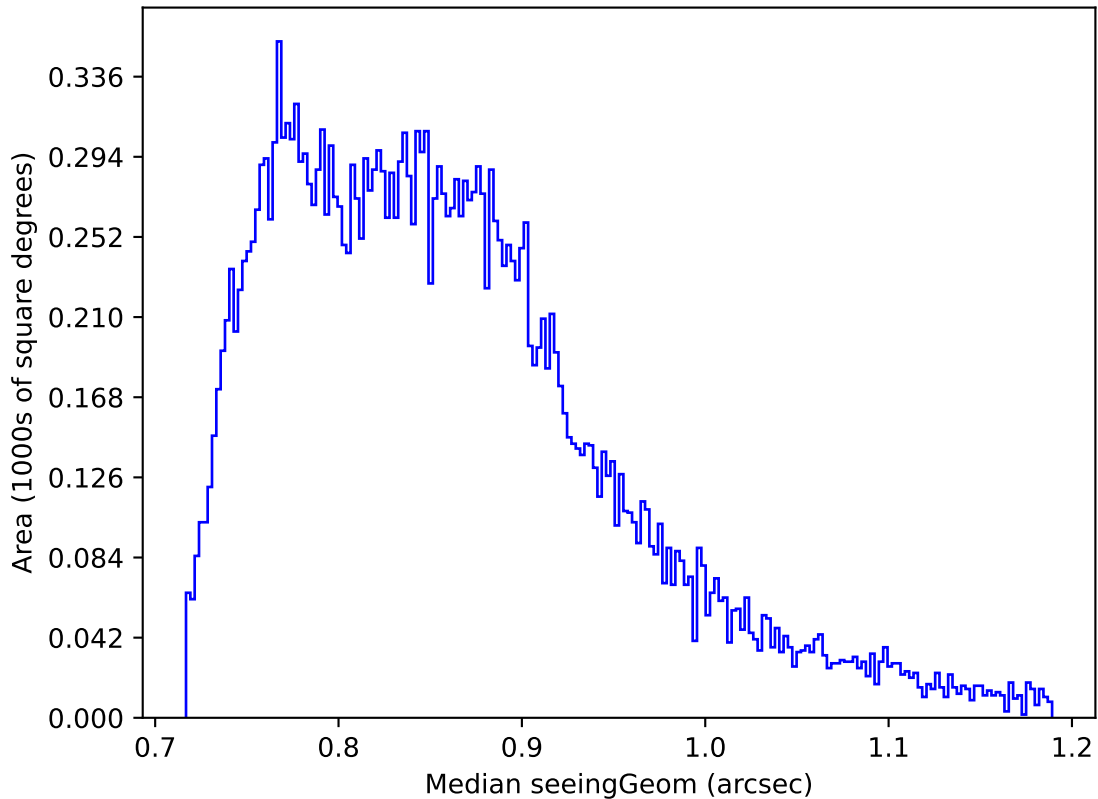
ddf_loaded_fl8_v3.4_10yrs Yr 1 all bands: Median seeingGeom
