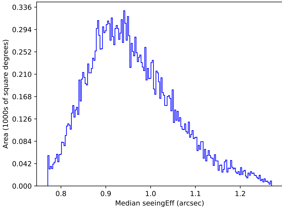
ddf_loaded_fl8_v3.4_10yrs Yr 1 y band: Median seeingEff
