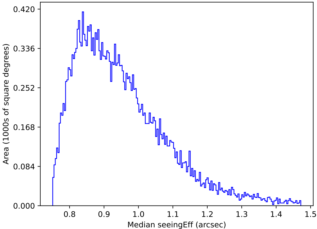
ddf_loaded_fl8_v3.4_10yrs Yr 1 i band: Median seeingEff
