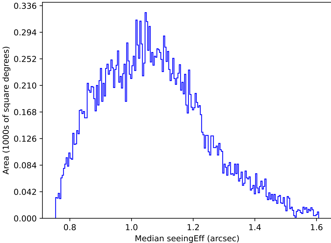
ddf_loaded_fl8_v3.4_10yrs Yr 1 g band: Median seeingEff
