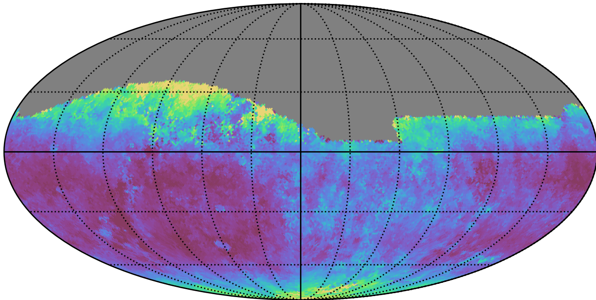
ddf_loaded_fl8_v3.4_10yrs Yr 1 all bands: Median seeingEff
