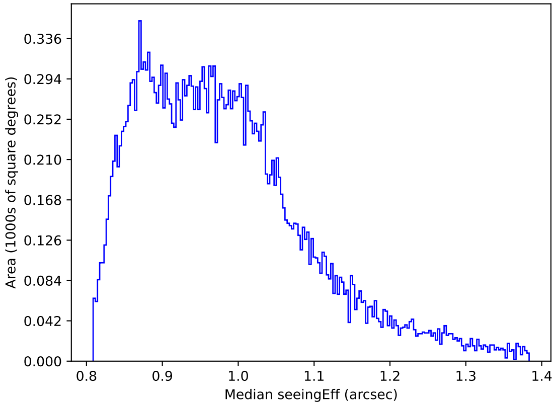
ddf_loaded_fl8_v3.4_10yrs Yr 1 all bands: Median seeingEff
