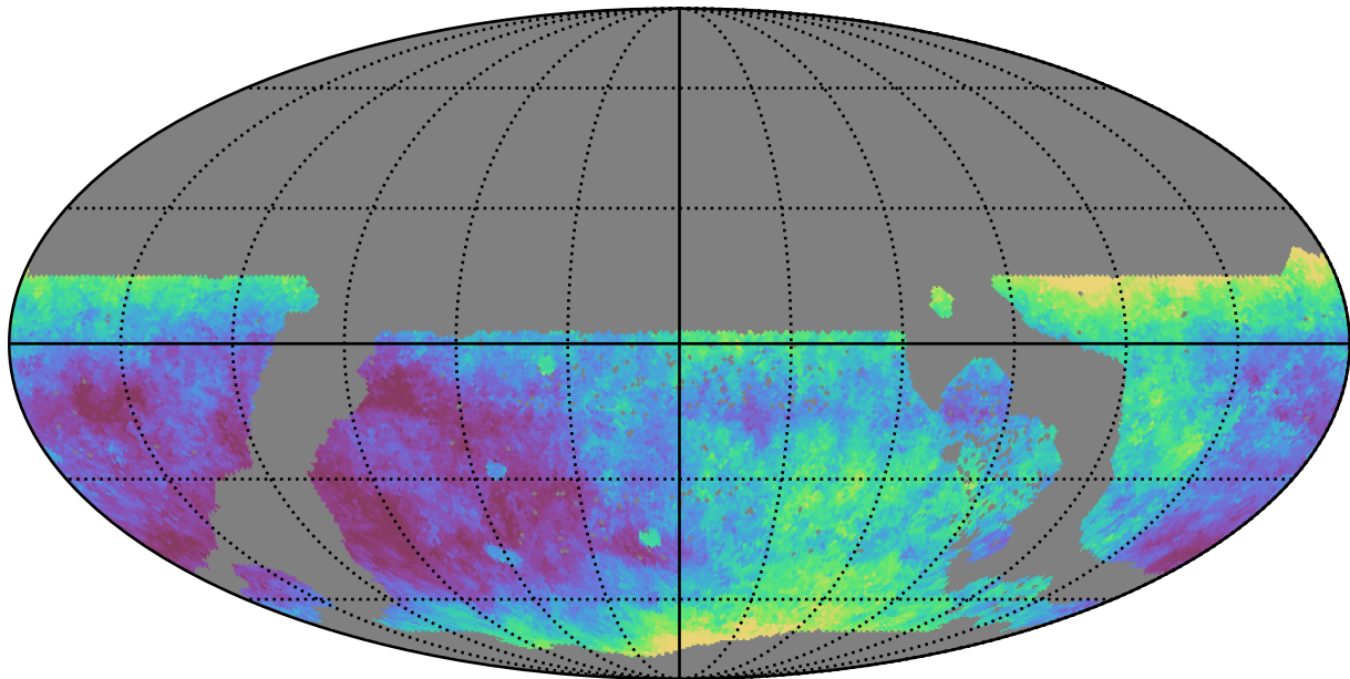
ddf_loaded_fl8_v3.4_10yrs WFD z band: Median seeingEff
