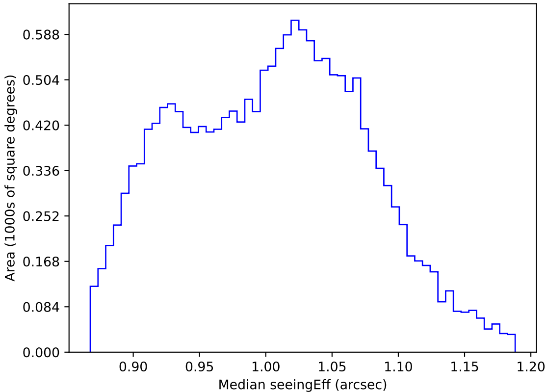
ddf_loaded_fl8_v3.4_10yrs WFD z band: Median seeingEff
