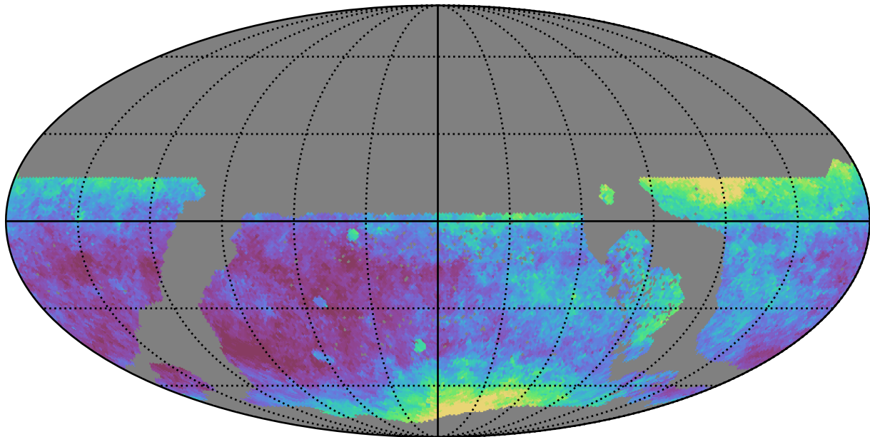
ddf_loaded_fl8_v3.4_10yrs WFD y band: Median seeingEff
