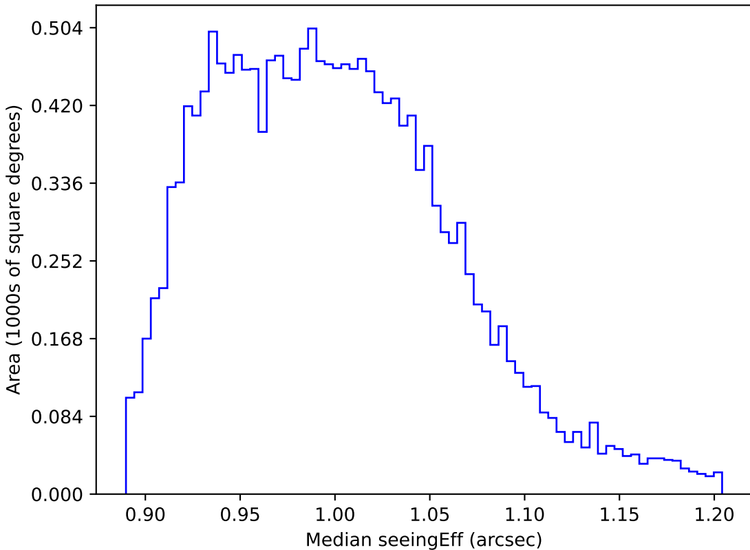
ddf_loaded_fl8_v3.4_10yrs WFD y band: Median seeingEff
