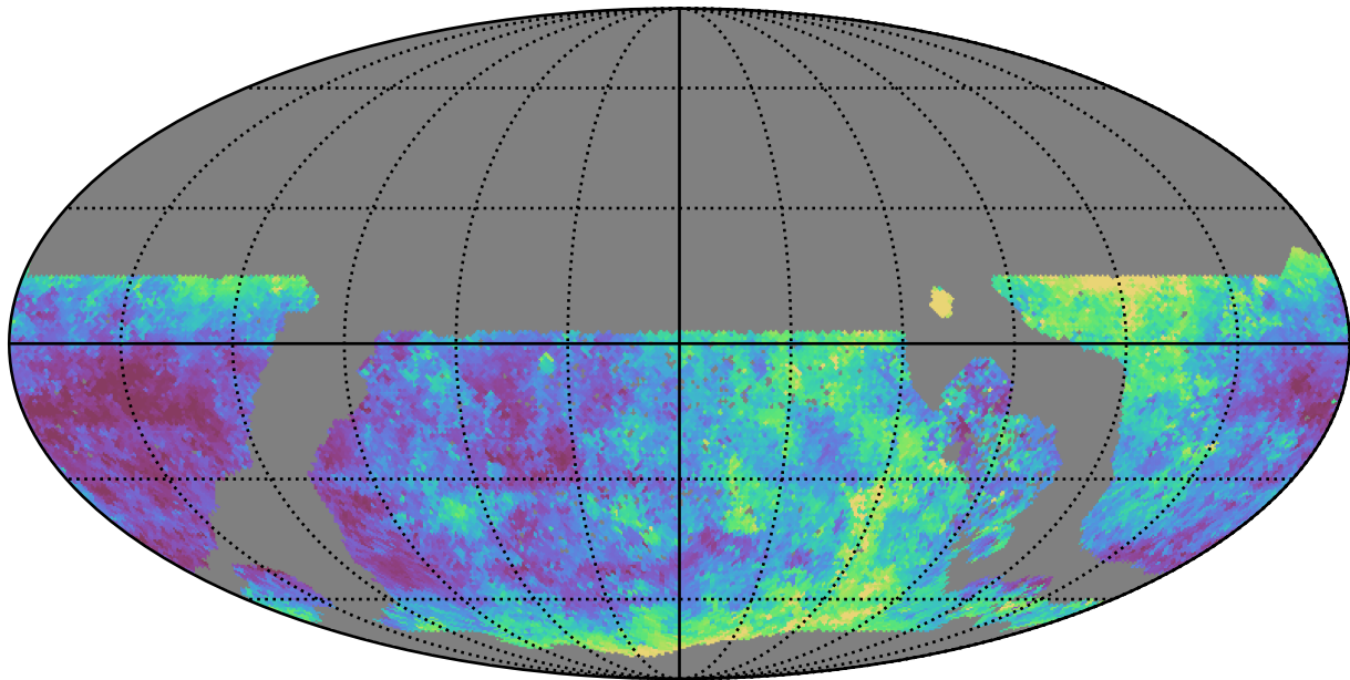
ddf_loaded_fl8_v3.4_10yrs WFD u band: Median seeingEff
