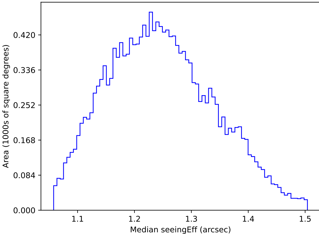
ddf_loaded_fl8_v3.4_10yrs WFD u band: Median seeingEff
