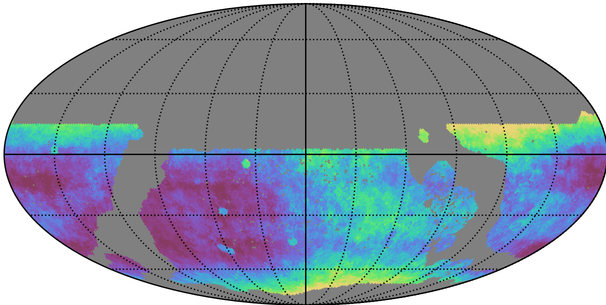
ddf_loaded_fl8_v3.4_10yrs WFD r band: Median seeingEff
