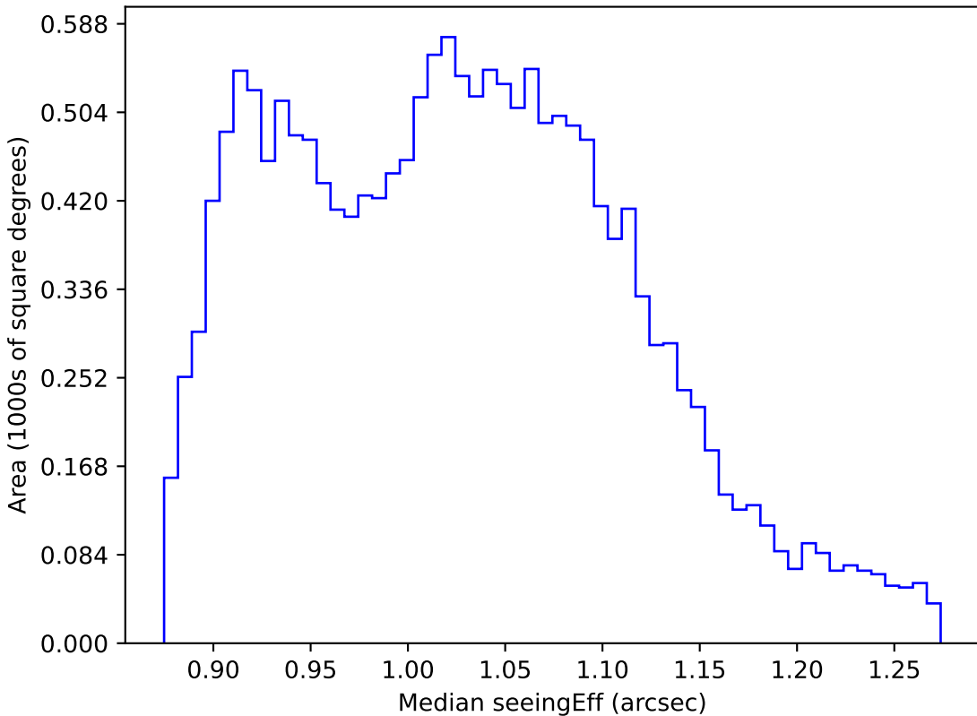
ddf_loaded_fl8_v3.4_10yrs WFD r band: Median seeingEff
