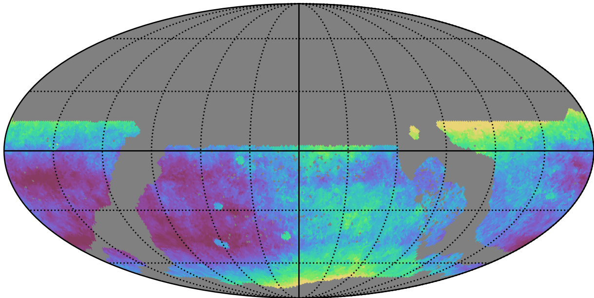
ddf_loaded_fl8_v3.4_10yrs WFD i band: Median seeingEff
