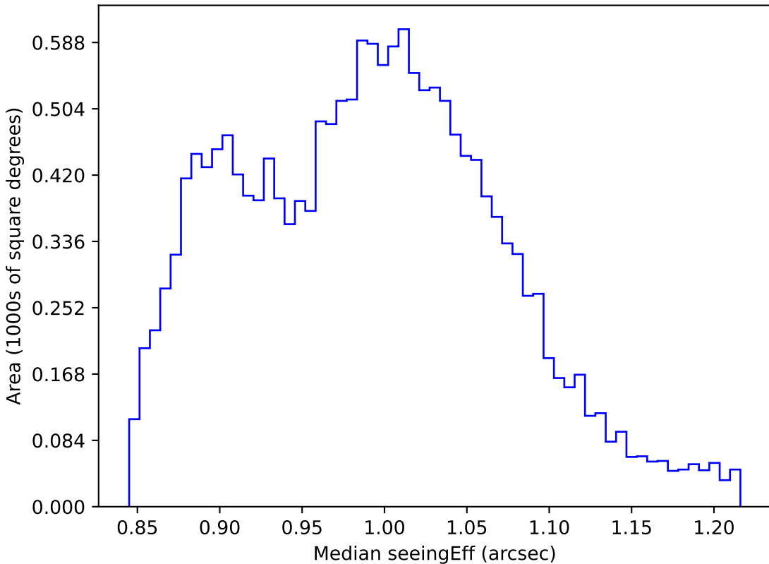
ddf_loaded_fl8_v3.4_10yrs WFD i band: Median seeingEff
