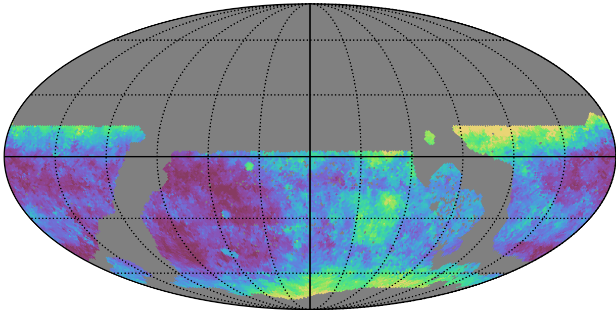
ddf_loaded_fl8_v3.4_10yrs WFD g band: Median seeingEff
