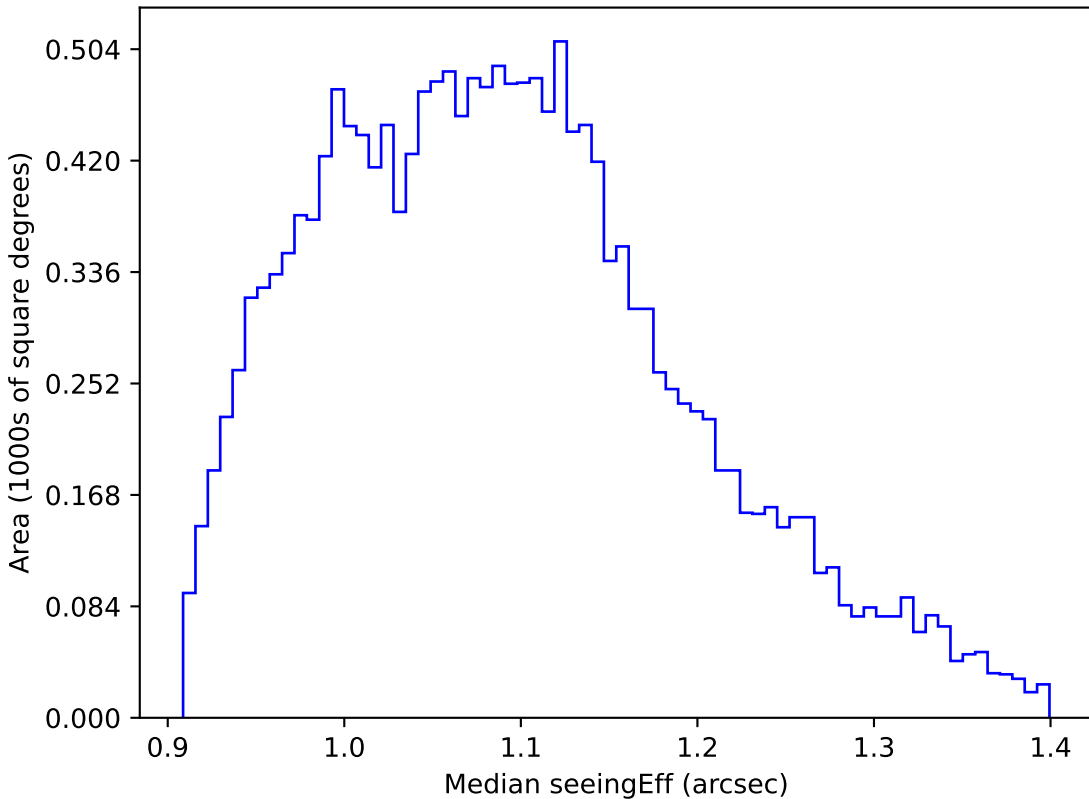
ddf_loaded_fl8_v3.4_10yrs WFD g band: Median seeingEff
